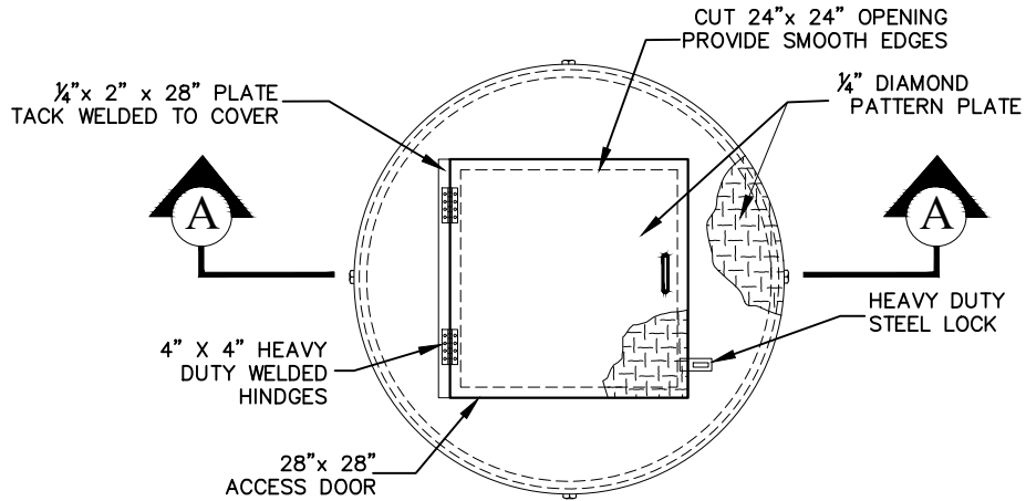
TOP VIEW OF COVER
